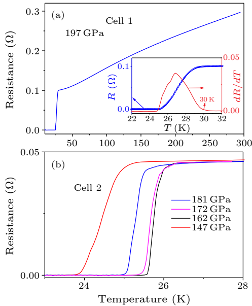
Fig. 1. (a) Temperature dependence of resistance for sample A (cell 1) measured at 197 GPa. The inset is the enlarged view of resistance curve and its temperature derivative to show the superconducting transition. (b) The superconducting transition curves for sample B (cell 2) measured at different released pressures.
