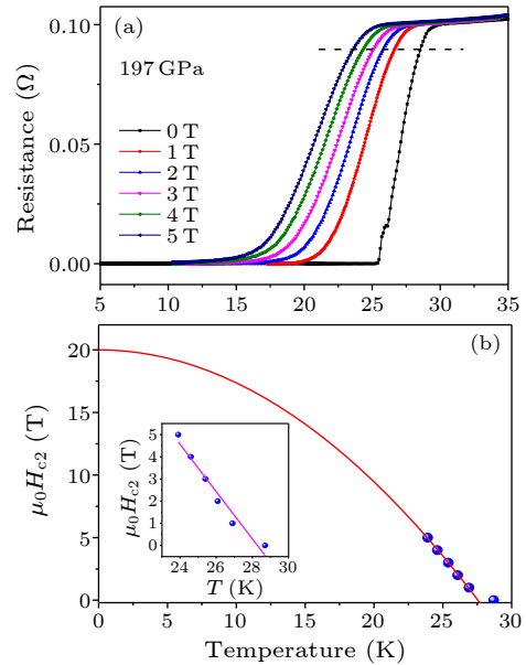
Fig. 2. (a) Superconducting transition for sample A (cell 1) measured at 197 GPa and different magnetic fields. (b) The upper critical magnetic field \mu_0 H_{c2}(T) versus T_c . The red line is the fitting via the Ginzburg–Landau (GL) theory. The inset shows the linear fitting for the \mu_0 H_{c2}(T) data.
