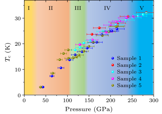
Fig. 4. Phase diagram of superconducting transition temperature T_c and crystal structure versus pressure for Sc. The measured results on all the five samples show consistent trends.
