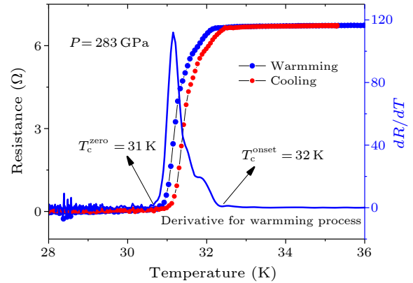
Fig. 2. The resistance curves measured at 283 GPa in both cooling and warming processes, where the derivative of the resistance with respect to temperature, dR/dT , for the warming process is plotted to clearly show the T_c^{\text{onset}} and T_c^{\text{zero}} .
