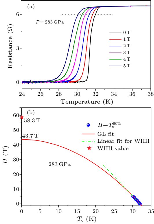
Fig. 3. (a) Temperature dependence of the electrical resistance of Sc metal measured at different magnetic fields under fixed pressure of 283 GPa. The dashed line marks the 90% of the normal state resistance. (b) Upper critical field \mu_0 H_{c2} versus temperature at 283 GPa. The Ginzburg-Landau (GL) fit for the H_{c2} (T) is shown by the solid lines. The star symbol represents the H_{c2} (0) values calculated via the Werthamer-Helfand-Hohenberg (WHH) model.
