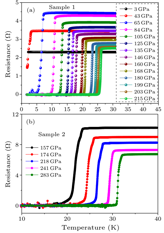
Fig. 1. Temperature dependence of the electrical resistance of elemental Sc metal measured at high pressures for (a) sample 1 and (b) sample 2.
