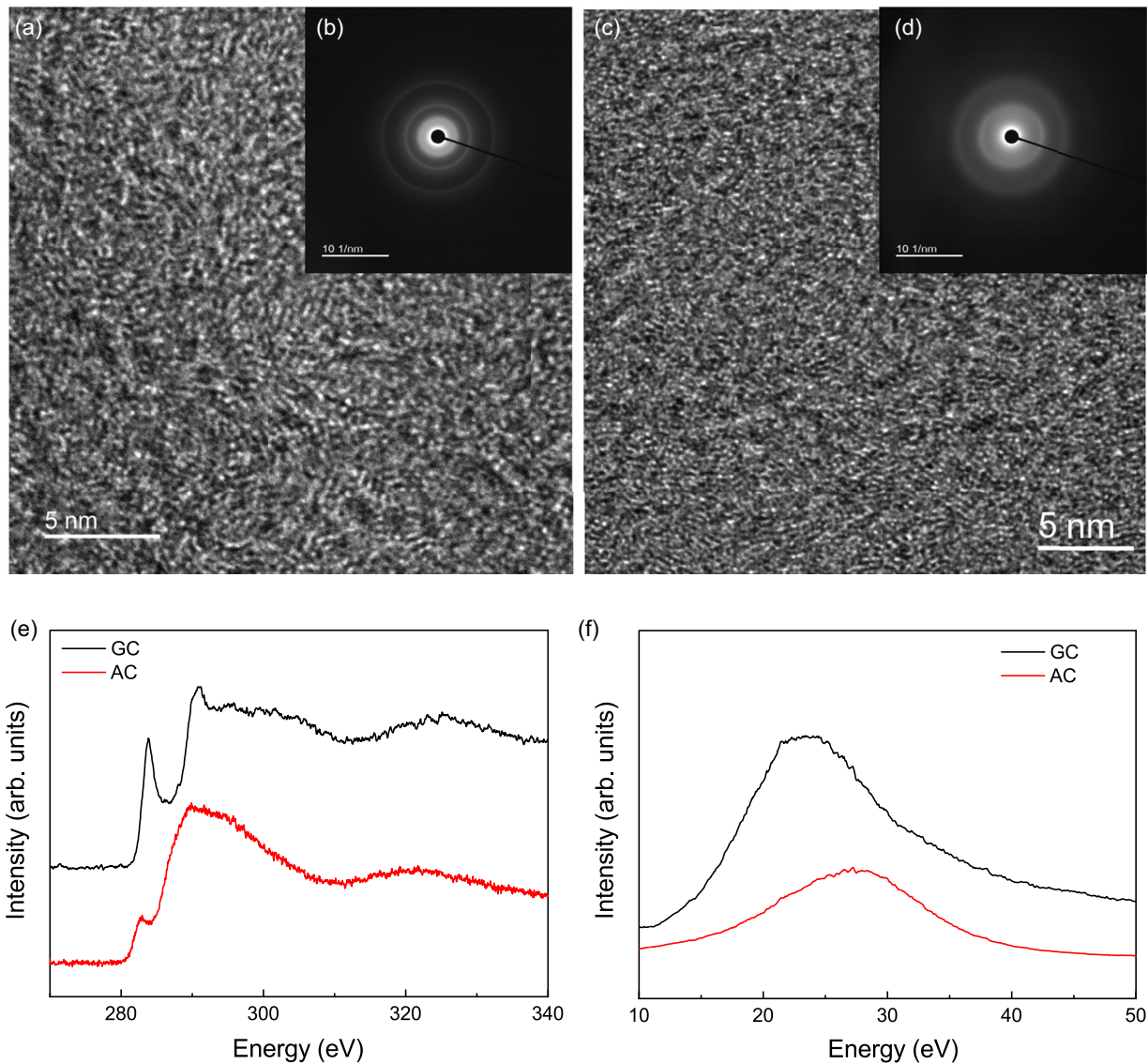
FIG. 6. TEM studies of the recovered sample. HRTEM image (a) and selected area electron diffraction (SAED) image (b) of GC; HRTEM (c) and SAED images (d) of the recovered sample AC. The scale bars in (a), (c) represent 5 nm. (e) Carbon K -edge EELS of GC (black) and the recovered sample AC (red). (f) The plasmon peak of GC (black) and the recovered sample AC (red).
