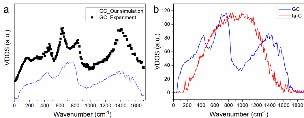
Figure S2 a. Experimental and calculated vibrational DOS of GC. The simulated VDOS for glassy carbon aligns well with the experimental data from [32]. b. Calculated vibrational DOS of GC and ta-C (with \sim 80\% \text{sp}^3 bonding). The VDOS profile for ta-C is consistent with prior simulations employing the Gaussian approximation potential model [33].
