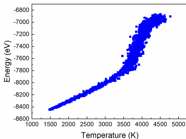
Figure S1 Potential energy as a function of temperature during the quenching process of liquid carbon in NVT ab initio MD simulation.
